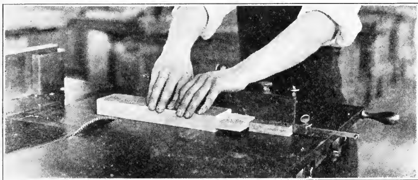
FIG. 167. SAWING TENON—SECOND END.
